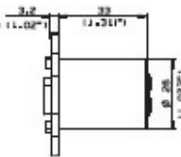
Internal cylinder
